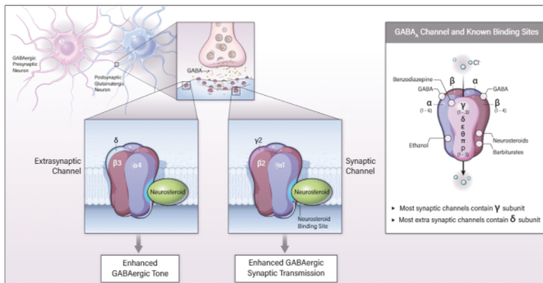
Figure 12. Mechanism of action of neurosteroid positive allosteric modulators (PAMs) of synaptic and extrasynaptic GABA A receptors. Neurosteroid PAMs can bind to and activate both synaptic and extrasynaptic GABA A receptors via an allosteric site distinct from the GABA and benzodiazepine binding sites. This potentiates the action of both phasic and tonic inhibitory neurotransmission mediated by GABA A receptors, leading to decreased neuronal excitability. ETX-155 is an investigational neurosteroid with dual potency at synaptic and extrasynaptic GABA A receptors.
